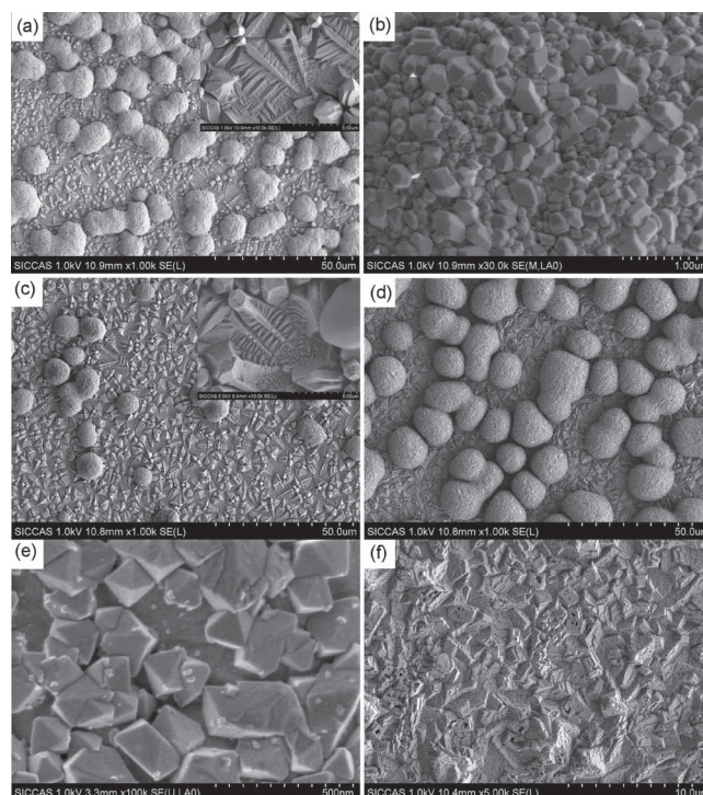
Figure 2. SEM images of (a) Cu/Cu 2 O-5.0-20, (b) the surface of spheres in Cu/Cu 2 O-5.0-20, (c) Cu/Cu 2 O-5.4-20, (d) Cu/Cu 2 O-5.4-60, (e) the spheres' surface of Cu/Cu 2 O-5.4-60, (f) Cu 2 O-5.8-20. The inset images in (a,c) shows the corresponding morphology at higher resolution. The scale bars of the insets are both 5 μm.
